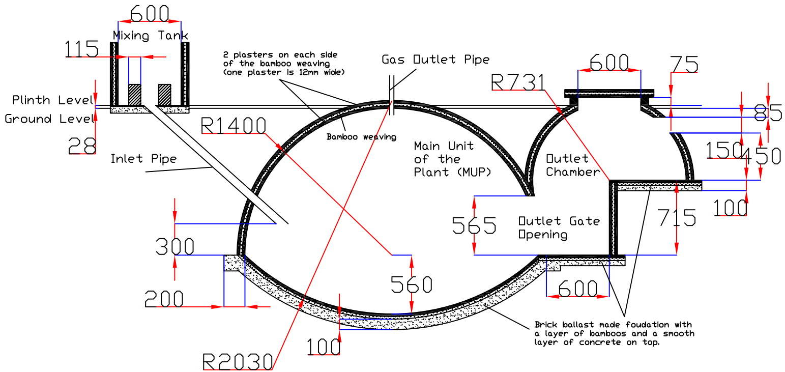
Sectional Elevation
